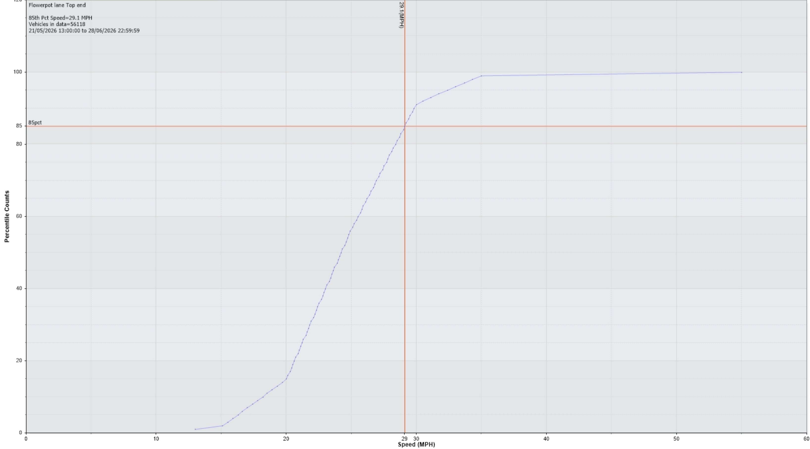
Percentile Counts Vs. Speed for [Flowerpot lane Top end : Incoming]
