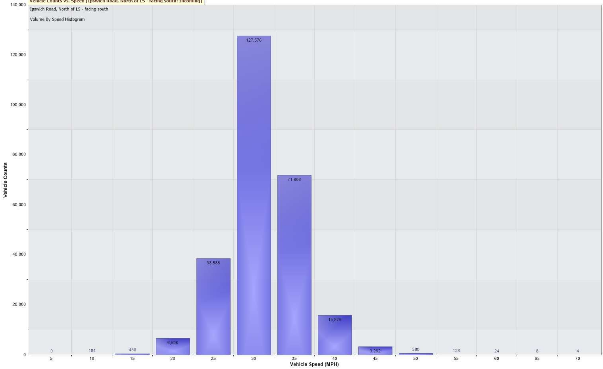
Vehicle Counts Vs. Speed [Ipswich Road, North of LS - facing south: Incoming]
